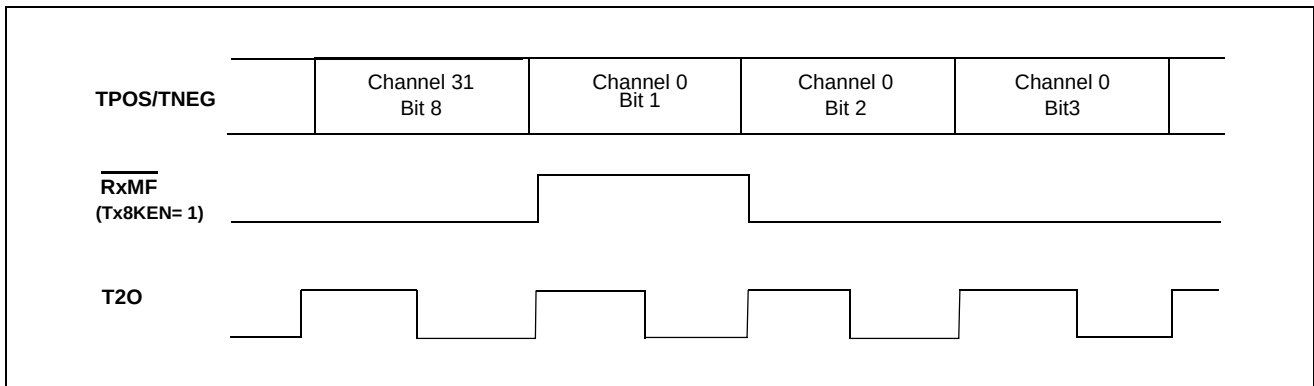
Figure 64 - Receive Multiframing Timing with TX8KEN Set
